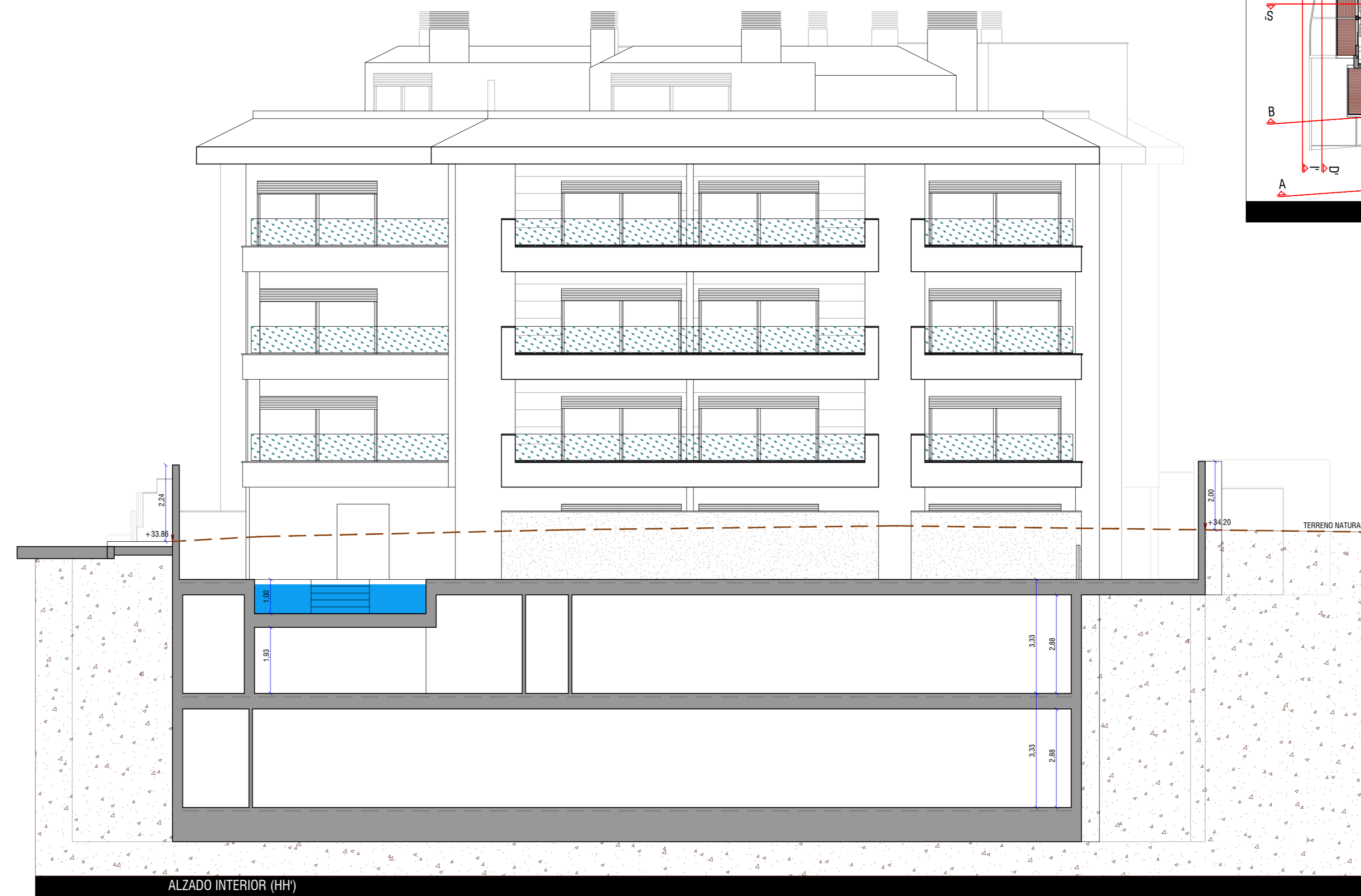
ALZADO INTERIOR (HH)
