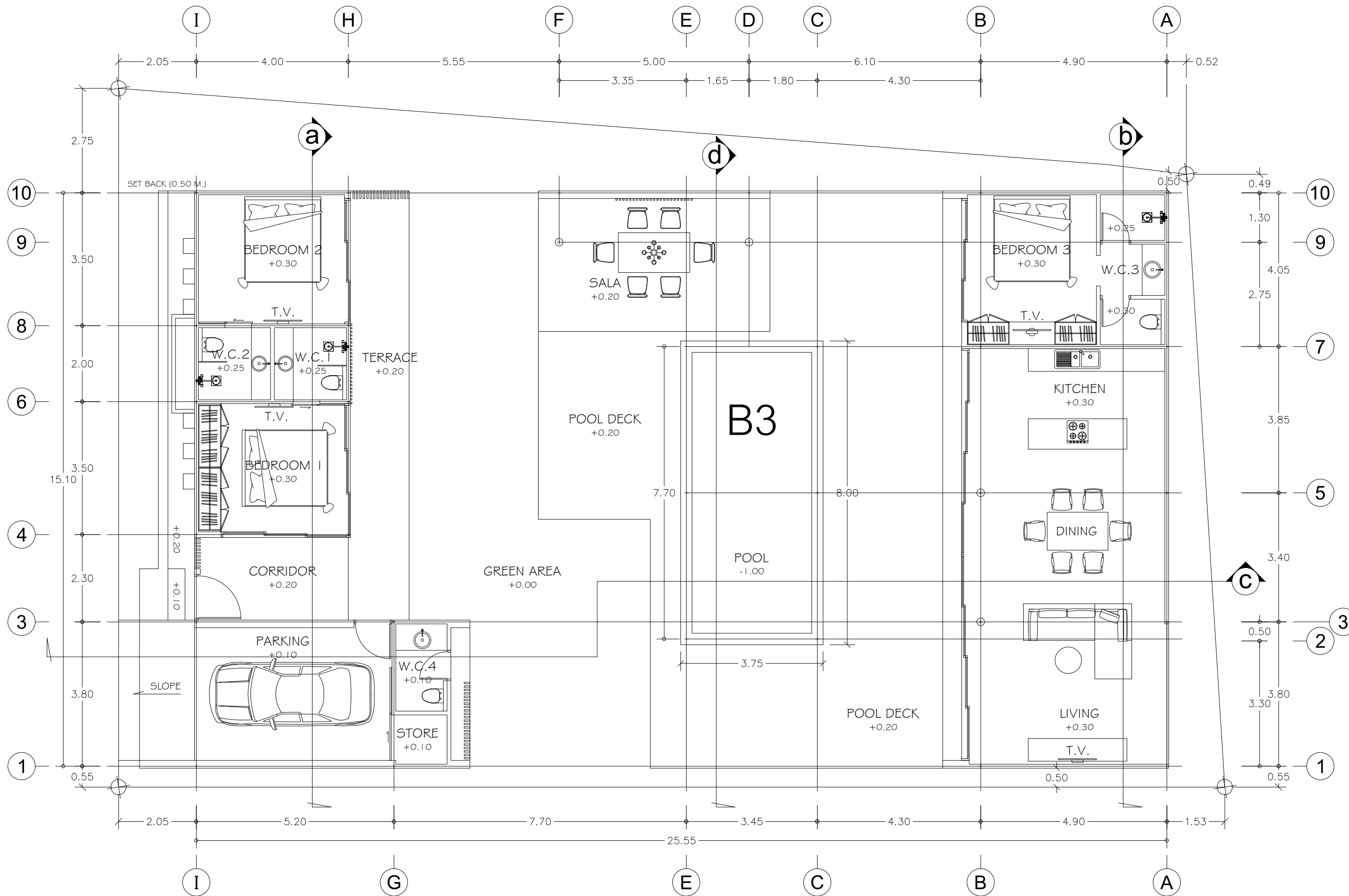
GROUND FLOOR PLAN PLOT B I SCALE 1 : 100
