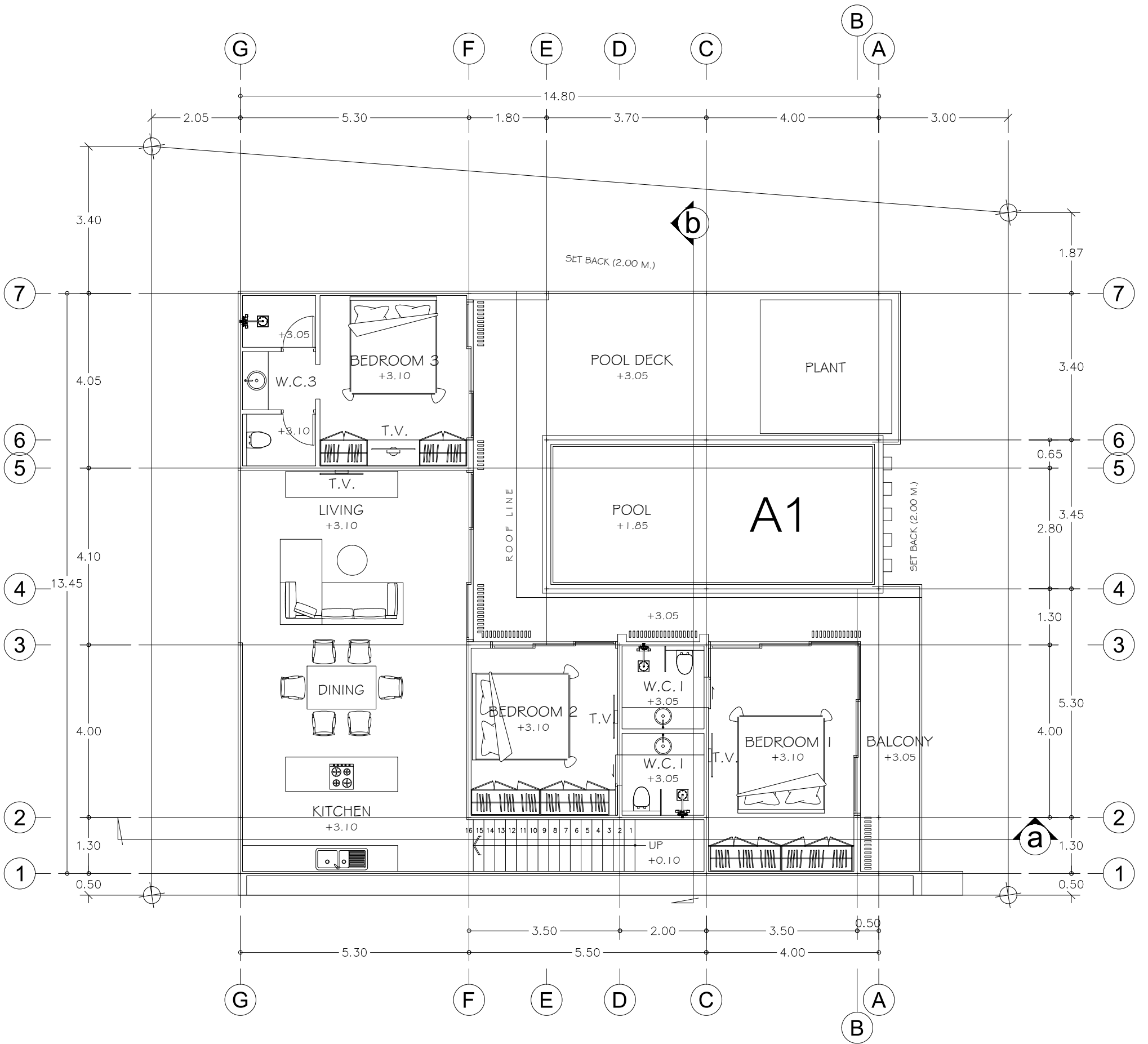
UPPER FLOOR PLAN PLOT A1 SCALE 1:100
