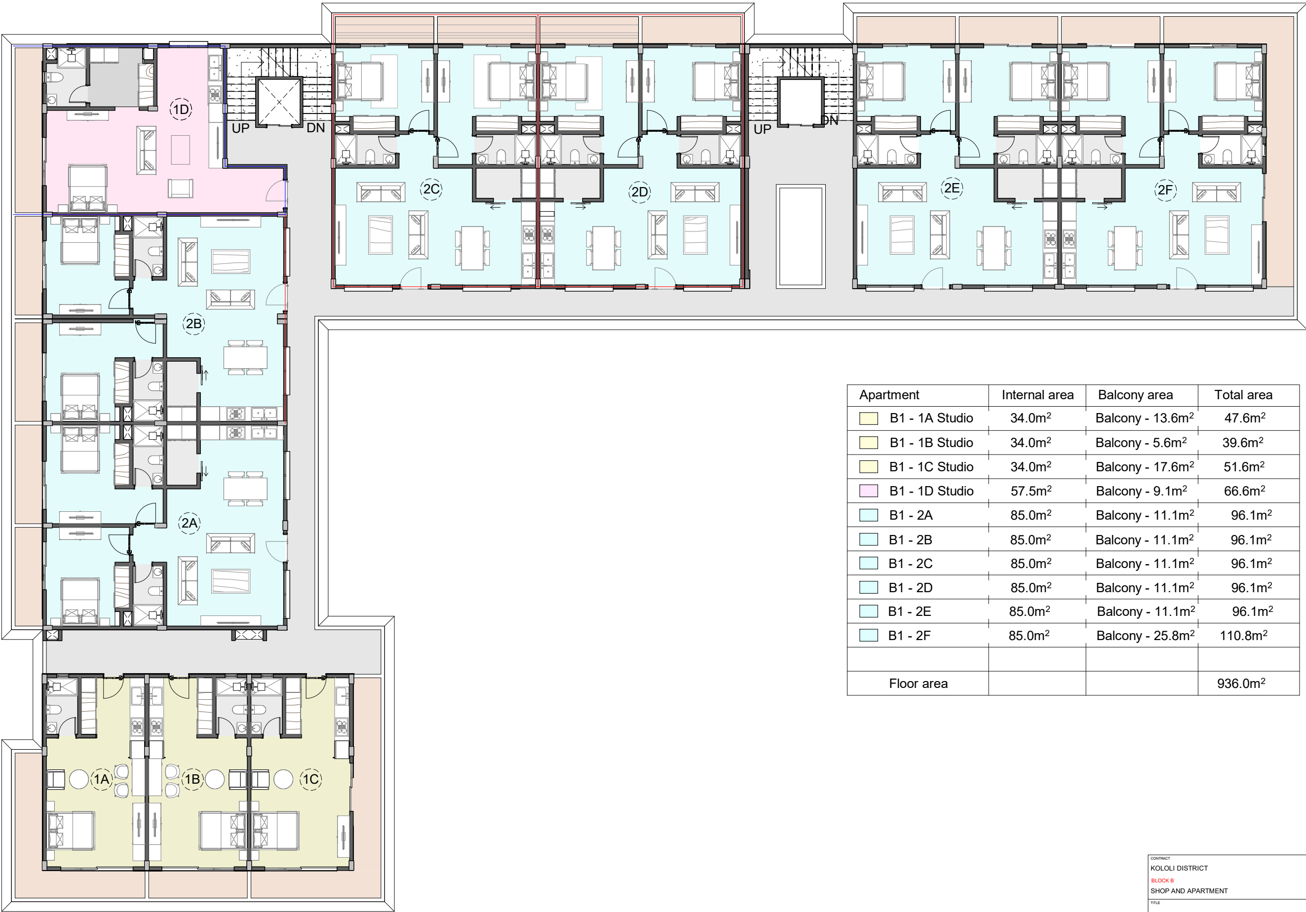
1 LEVEL 1 DEPARTMENT LAYOUT 1 : 155
