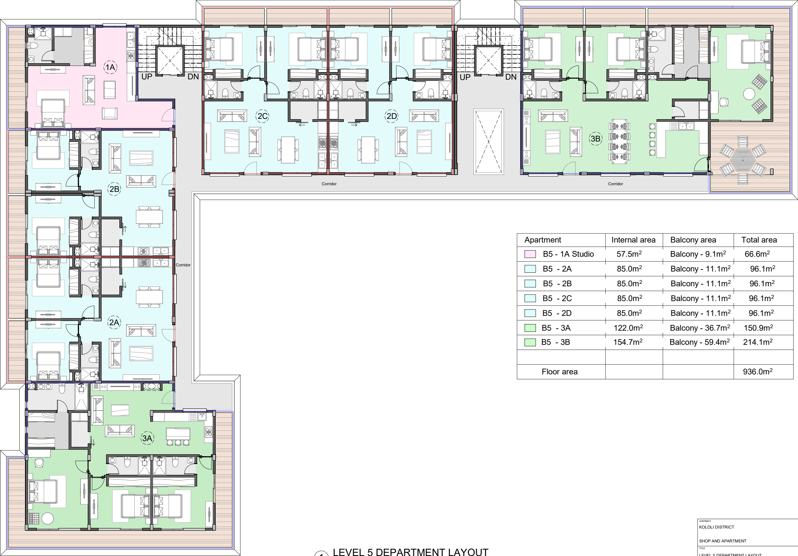
1 LEVEL 5 DEPARTMENT LAYOUT 1 : 155
