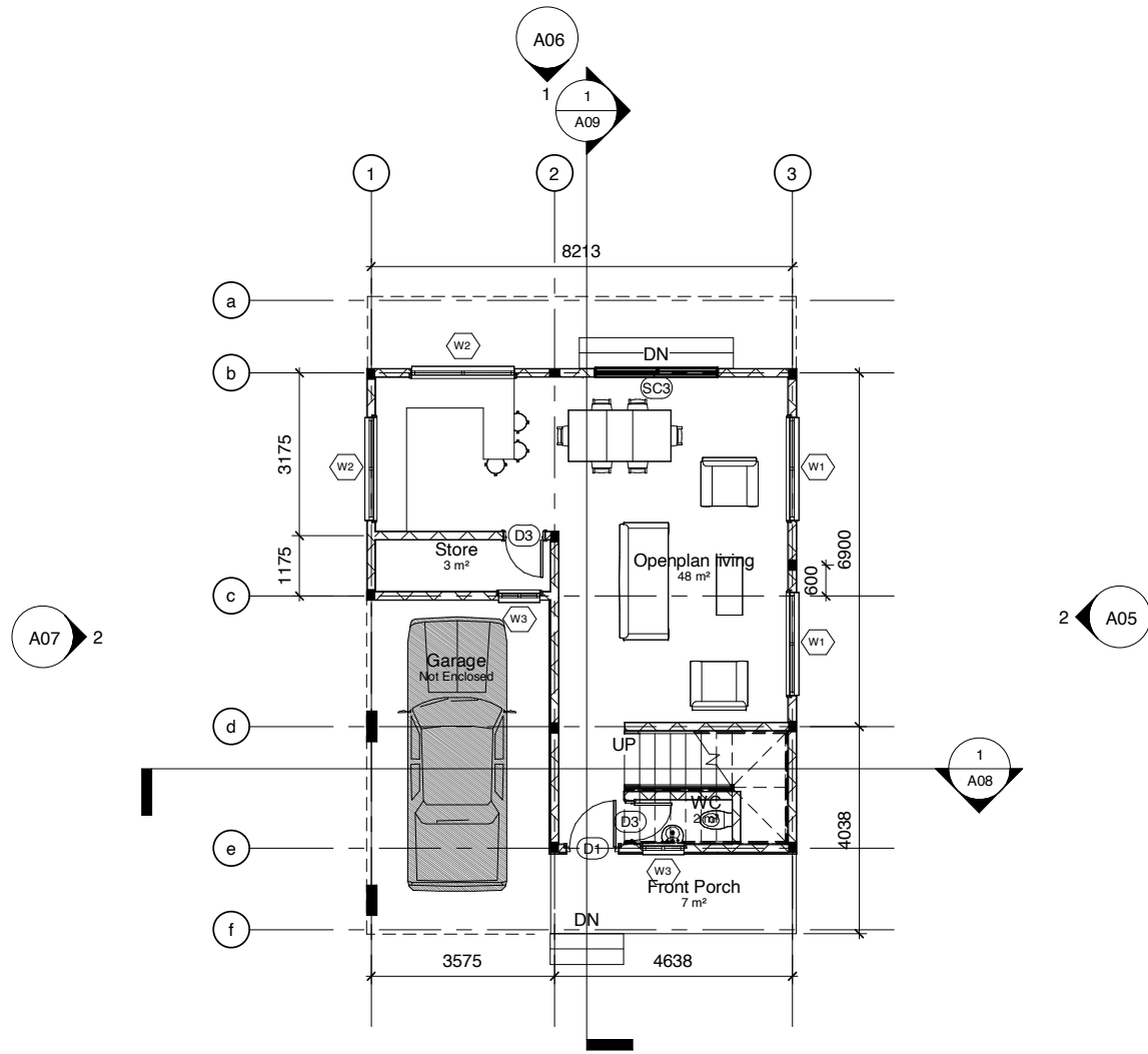
1 Ground Floor 1 : 100
