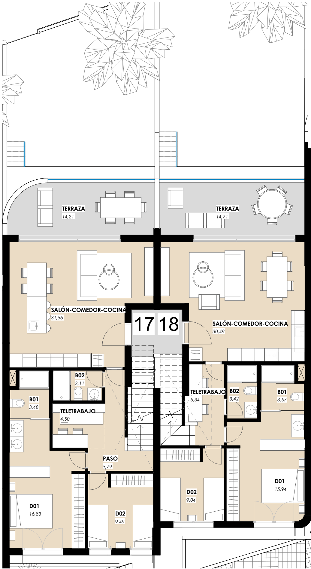
VIVIENDA 17-18_PLANTA PRIMERA/ APARTMENT 17-18_TOP FLOOR
